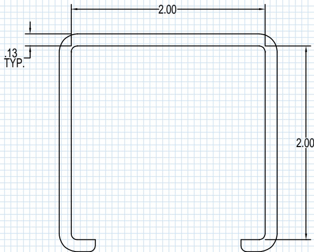
SPX 1063588 CAT CC-200-200 Fits 2" x 2" Bar
