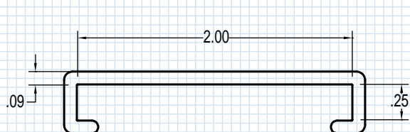
SPX 1002639 CAT CB-025-200 Fits 1/4" x 2" Bar or AR-60 Aluminum Rail
