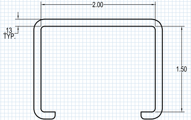
SPX 1012709 CAT CC-150-200 Fits 1/2" x 2" Bar
