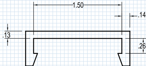
SPX 1952103 CAT PC-025-150 Fits 1/4" x 1 1/2" Bar
