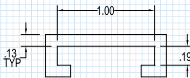
SPX 1760731 CAT CC-019-100 Fits 3/16" x 1" Bar
