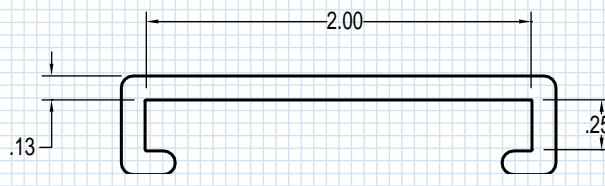
SPX 1012738 CAT CC-025-200 Fits 1/4" x 2" Bar or AR-60 Aluminum Rail
