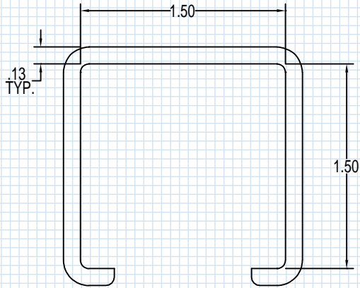
SPX 1022866 CAT CC-150-150 Fits 1/2" x 1/2" Bar
