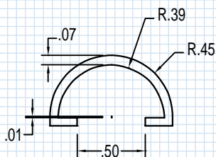
SPX 1851314 THIN WALL For 3/4" Half Bar
